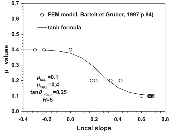
Fig. 6. Relationship between \mu values and the local slope for Aulta path (Bartelt and Gruber, 1997).
