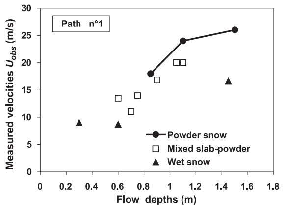
Fig. 4. Relationship between the height and the velocity of the avalanche at the measurement point.
