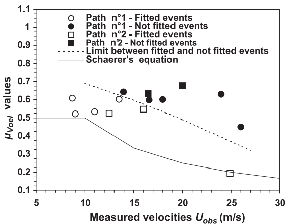
Fig. 9. Results of the Voellmy-like model fitting on Col du Lautaret site data.
