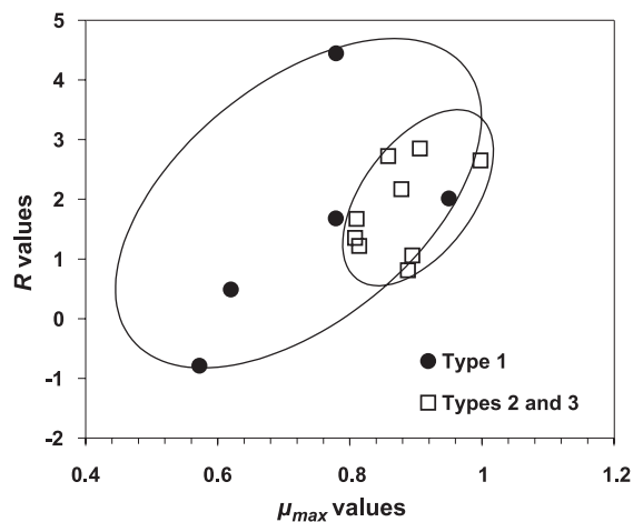
Fig. 10. Independence between the two fitting parameters of the Generalized Voellmy-like model ( \mu_{min} = 0.1 - \tan\theta_{moy} = 0.6 ).
