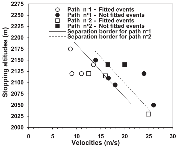
Fig. 8. Separation between fitted events and nonfitted events for the Voellmy-like model.
