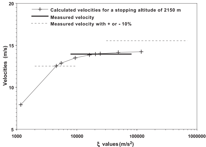
Fig. 5. Results of the Voellmy-like model fitting for the event of 14/02/03 on Path 1, obtained for a fixed value of the stopping elevation.
