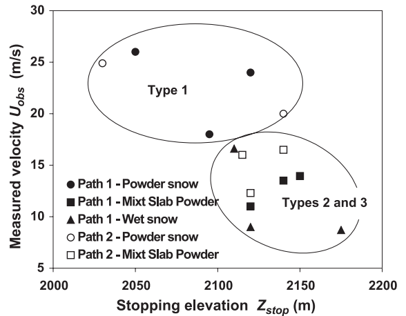
Fig. 3. Separation between Type 1 avalanches and Types 2 and 3 avalanches.
