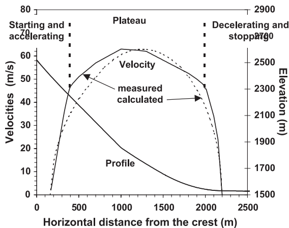
Fig. 7. Profile of the Aulta avalanche dynamic with measured velocities (Bartelt and Gruber, 1997) and velocities calculated with the modified Coulomb-like model (dashed-line) ( \mu=0.4272 , k=1.075 ).
