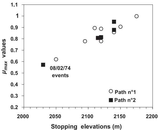
Fig. 11. Variation of \mu_{\max} depending on the stopping elevation for Generalized Voellmy-like model.
