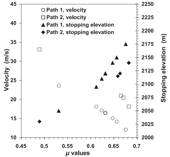
Fig. 12. Relationship between the \mu values of the modified Coulomb-like model and the stopping elevations and velocities for the Lautaret paths.
