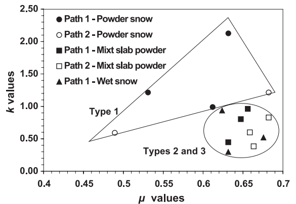
Fig. 13. The internal parameters obtained by fitting the modified Coulomb-like model.
