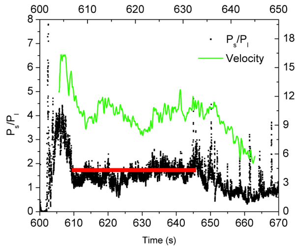
Fig. 10: Avalanche #20090003: Ratio P_s/P_l between pressure measured at the small sensors, P_s , and pressure measured at the large plate, P_l . The ratio in the wet-dense part is 1.7. Velocity, in green, is superimposed for easy comparison.
