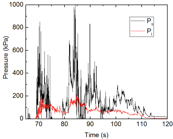
Fig. 4: Avalanche 7226: Comparison between impact pressures measured at the tower (black line, average between small sensors at 2.5 and 3.5 m above ground) and impact pressure measured at the small concrete wall with the 1 m 2 plate (red line).
