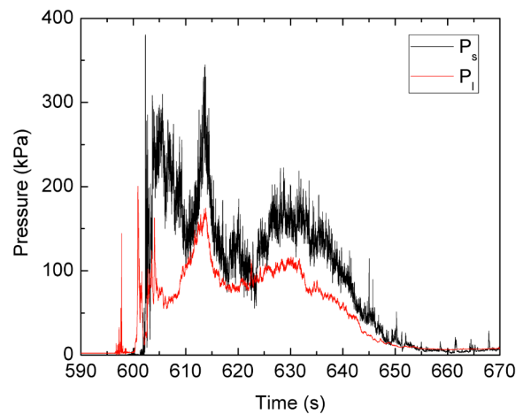
Fig. 7: Avalanche #20090003: Comparison between impact pressures measured at the tower (black line, average between small sensors at 2.5 and 3.5 m above ground) and impact pressure measured at the small concrete wall with the 1 m 2 plate (red line).
