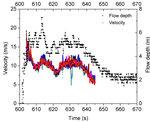
Fig. 8: Avalanche #20090003: Flow depth (black line) and average velocities (colored dots) measured at the tower between 2.5 and 3.5 m above ground.
